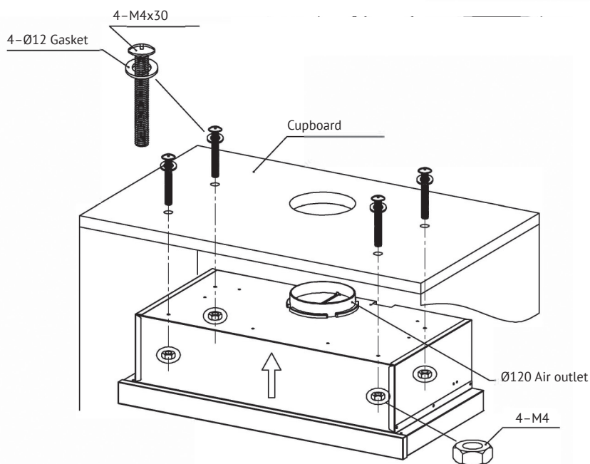
Installation diagram
