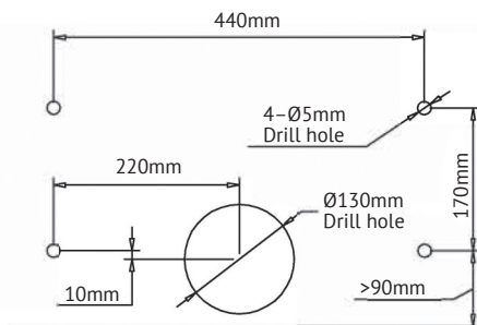
Drill size diagram
